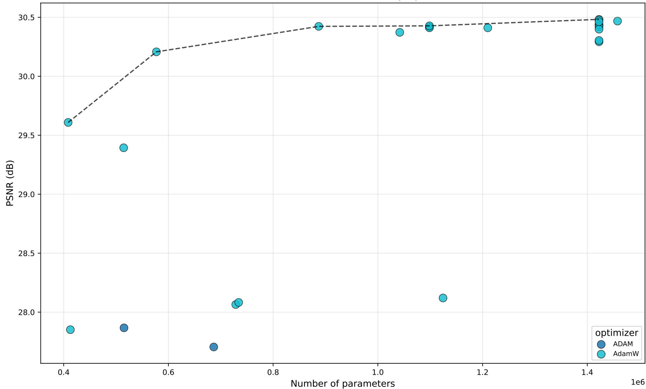
PSNR vs #Params — SwinT — by optimizer
